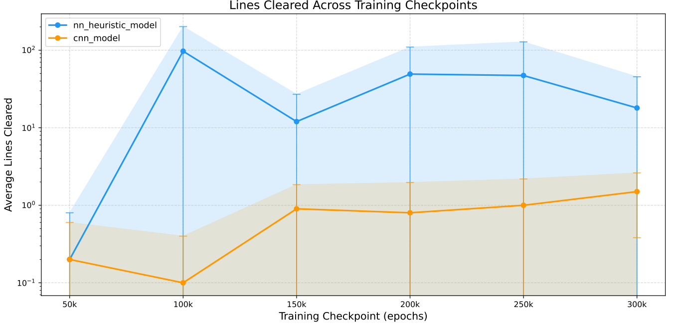
Figure 2: The average number of lines cleared by each model per game over 100 games at different training epochs.
